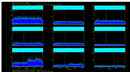
Figure 1: Dynamic spectrum of the water maser emission in S255IR-SMA1 in 2010 from
