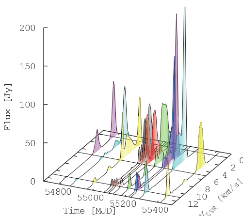
Figure 5: Dynamic spectrum of the water maser emission in S255IR-SMA1 in 2010 from
