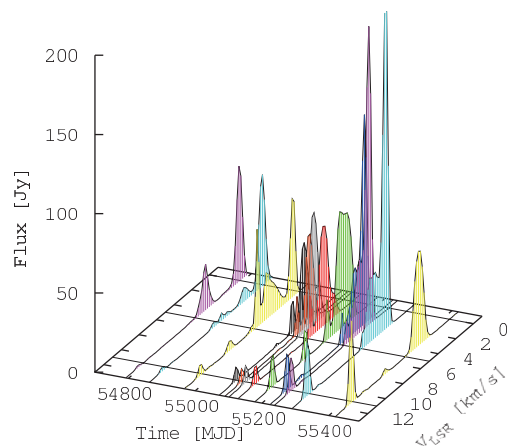
Figure 7: Dynamic spectrum of the water maser emission in S255IR-SMA1 in 2010 from
