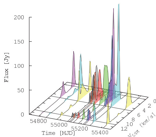
Figure 4: Dynamic spectrum of the water maser emission in S255IR-SMA1 in 2010 from
