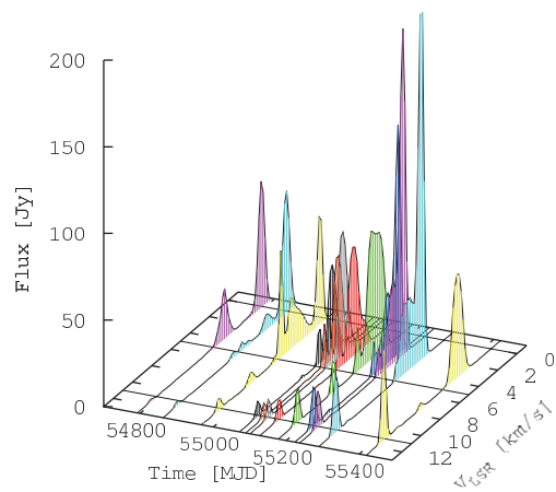
Figure 1: Dynamic spectrum of the water maser emission in S255IR-SMA1 in 2010 from
