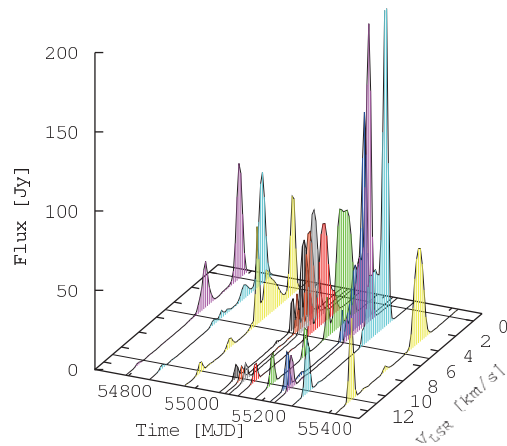
Figure 3: Dynamic spectrum of the water maser emission in S255IR-SMA1 in 2010 from
