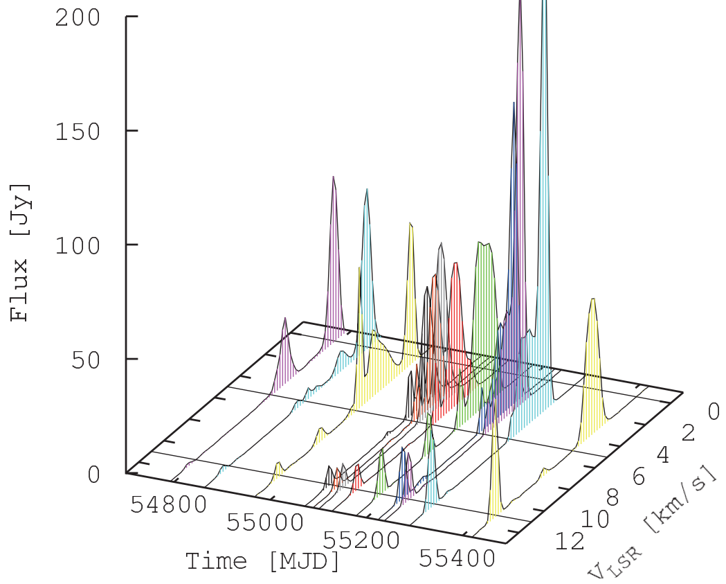
Figure 16: Dynamic spectrum of the water maser emission in S255IR-SMA1 in 2010 from
