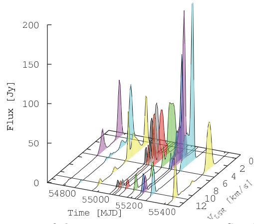
Figure 2: Dynamic spectrum of the water maser emission in S255IR-SMA1 in 2010 from
