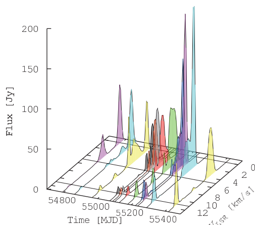
Figure 11: Dynamic spectrum of the water maser emission in S255IR-SMA1 in 2010 from
