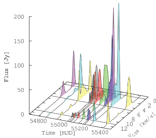
Figure 13: Dynamic spectrum of the water maser emission in S255IR-SMA1 in 2010 from Dynamic spectrum of the water maser emission in S255IR-SMA1 in 2010 from Dynamic spectrum of the water maser emission in S255IR-SMA1 in 2010 from Dynamic spectrum of the water maser emission in S255IR-SMA1 in 2010 from
