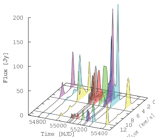
Figure 12: Dynamic spectrum of the water maser emission in S255IR-SMA1 in 2010 from
