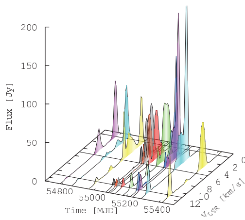
Figure 10: Dynamic spectrum of the water maser emission in S255IR-SMA1 in 2010 from
