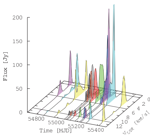
Figure 6: Dynamic spectrum of the water maser emission in S255IR-SMA1 in 2010 from
