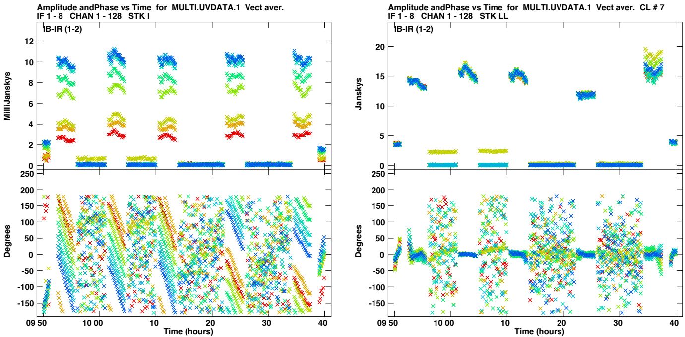
Figure 1: Visibility vs time plots (VPLOTs) of (Left) Uncalibrated data, and (Right) data calibrated using the automatic pipeline. Phases can be seen to align in both time and frequency for all sources (G85.411+0.002 and CEPA, and calibrators) and amplitudes agree across all BBCs and polarisations
